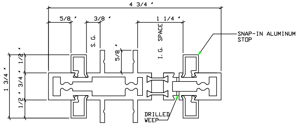
INTERIOR MULLION
